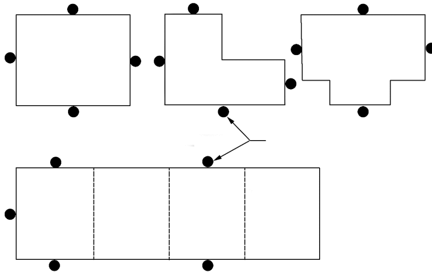
Figure 14 typically recommended locations for exterior pressure pickups
